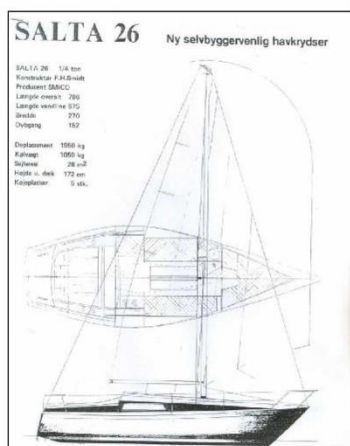
Rig of Salta 26
